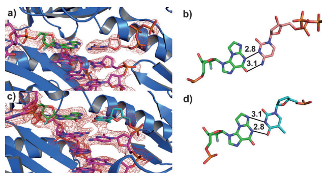
Figure 2. Crystal structures of Dpo4- N^2,3\text{-}\epsilon\text{G} -DNA complexes (Z = C in the template). a) Ternary complex of Dpo4 with dCTP and N^2,3\text{-}\epsilon\text{G} -containing duplex DNA, (Dpo4-1) and b) the orientation of the bases with proposed hydrogen-bonding mechanism (distances shown in Å). c) Binary complex of Dpo4 with ddT across from N^2,3\text{-}\epsilon\text{G} in the DNA duplex (Dpo4-3) and d) the orientation of the bases with proposed hydrogen-bonding mechanism. The quality of the data is demonstrated using non-biased omit electron density maps, displayed as red mesh, at 1.0 \sigma in (a) and (c). Colors of the atoms: O, red; N, blue; P, orange; F, gray.
